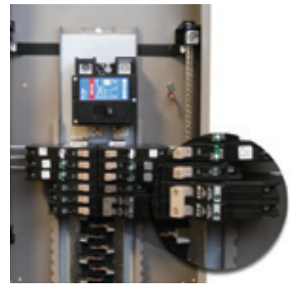
Internally mounted surge breaker option
